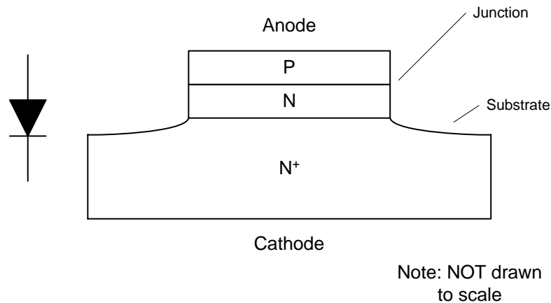
Figure 1 Varactor Diode Cross Section
