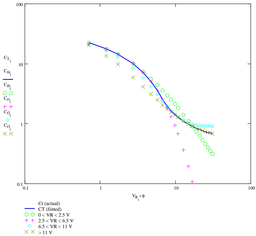
Figure 12 SMV1265-011 Piecewise C-V Curves
