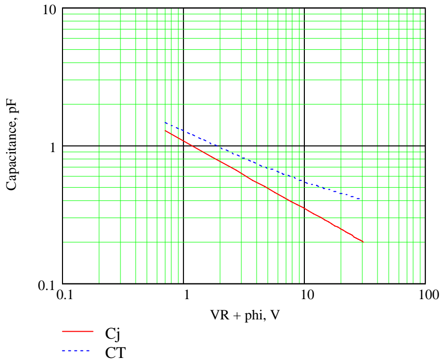
Figure 8 Junction and Total Capacitance versus V_R + \phi
