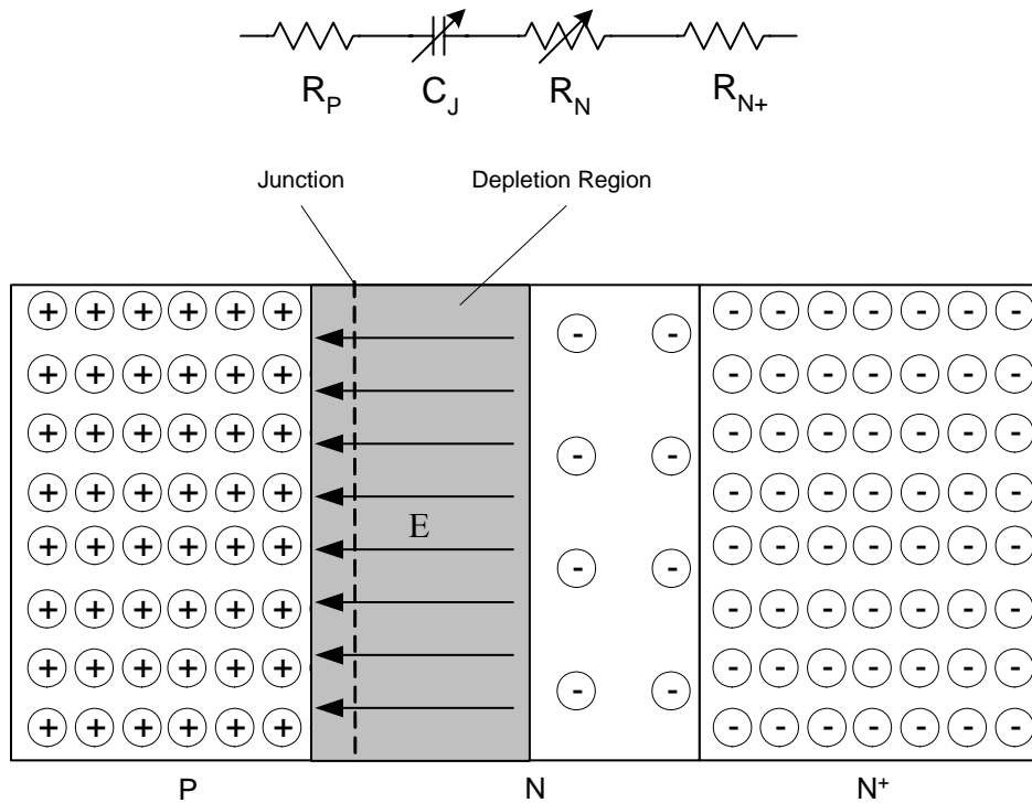
Figure 5 Varactor Simple Series Equivalent Circuit
