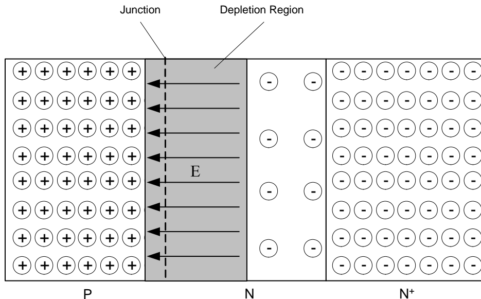
Figure 3 The Varactor Diode Junction and Depletion Region
