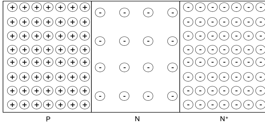
Figure 2 The Layers of a Varactor Diode
