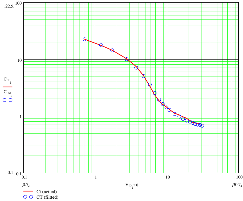
Figure 11 SMV1265-011 Actual and Fitted C_T vs. V_R + \phi
