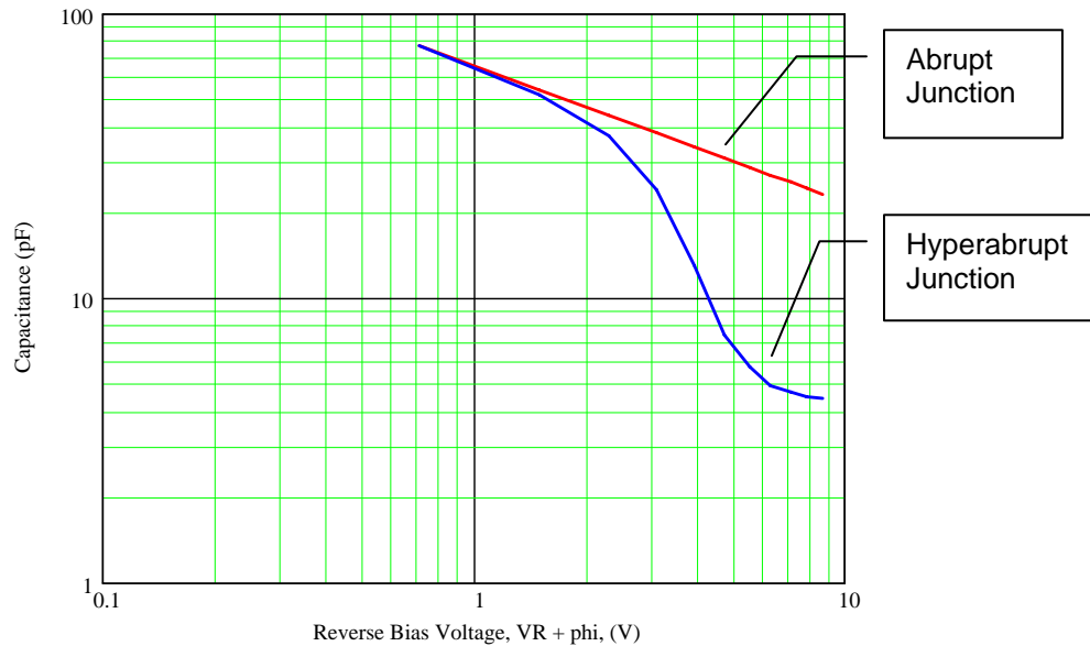
Figure 4 C_J vs. V_R for an Abrupt and a Hyperabrupt Varactor versus V_R + \phi
