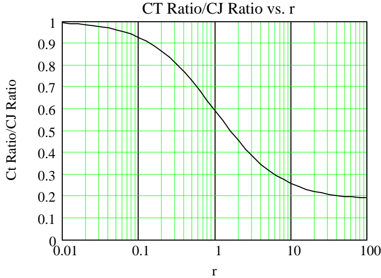
Figure 9 Total Capacitance Ratio Normalized to Junction Capacitance Ratio versus r
