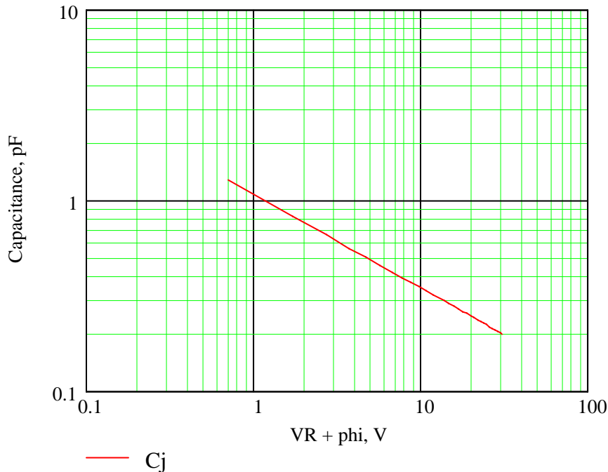
Figure 7 Junction Capacitance versus V_R + \phi
