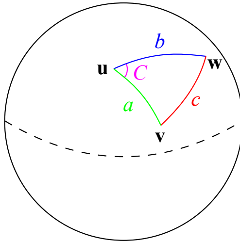
Figure 5.3: Spherical triangle solved by the law of cosines [2]
