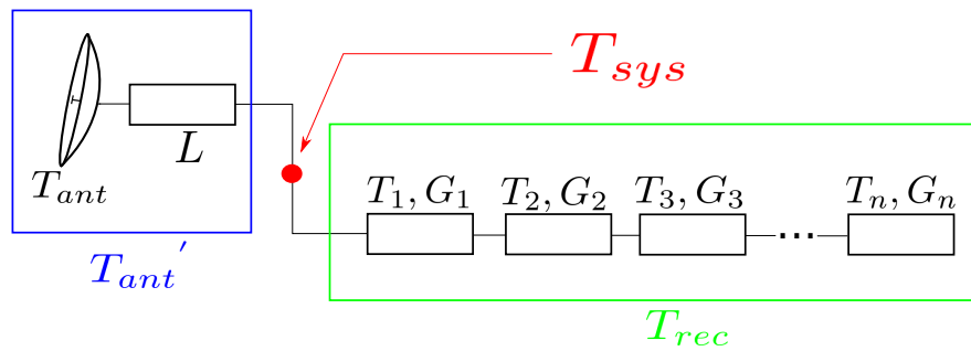
Figure 3.10: Reference point of system noise temperature
