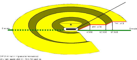
Improved TCF Envelope
