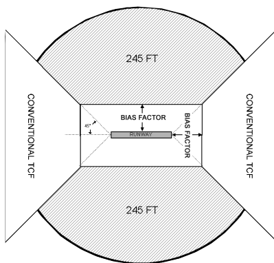
Improved TCF Envelope Plan View
